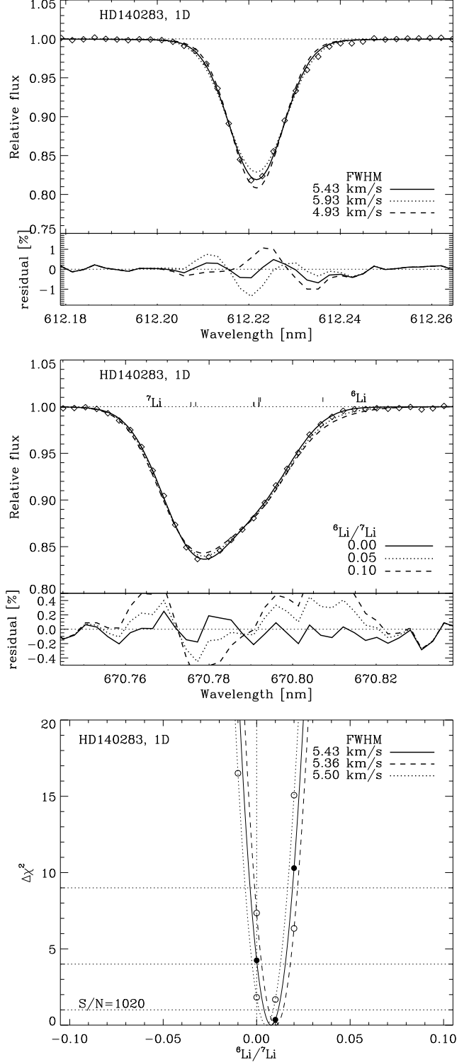
FIG. 9.— Upper panel: Observed Ca I 612.2 nm profile (rhombs) in HD 140283 together with the best fit theoretical 1D LTE profile (solid line). Also shown are the predictions with the macroturbulence \zeta_{\text{macro}} \pm 0.5 \text{ km s}^{-1} . The Gaussian FWHM is here the combination of \zeta_{\text{macro}} and the instrumental broadening; the profiles have also been convolved with a stellar rotation velocity of v_{\text{rot}} = 0.5 \text{ km s}^{-1} . Middle panel: Computed Li I 670.8 nm profile for three different values for {}^6\text{Li}/{}^7\text{Li} (0.00, 0.05 and 0.10) shown together with the observed line (rhombs). In each case, the Li abundance, wavelength shift and continuum level have been allowed to vary. The location of the various {}^7\text{Li} and {}^6\text{Li} components are indicated. Lower panel: Resulting \Delta\chi^2 for the combined Gaussian of the mean \zeta_{\text{macro}} and instrumental broadening; also shown are the cases for \zeta_{\text{macro}} \pm \Delta\zeta_{\text{macro}} . In this star, no significant detection of {}^6\text{Li} can be claimed.
